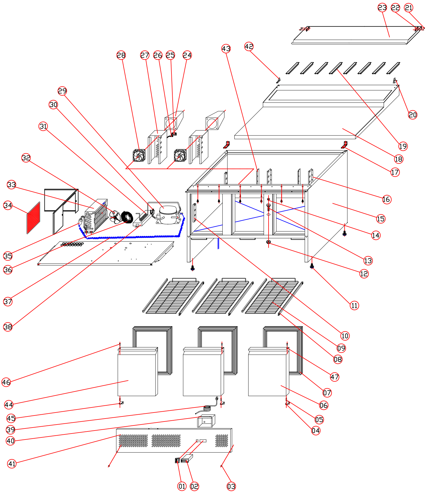
EXPLODED VIEW OF PS300GN1/6
